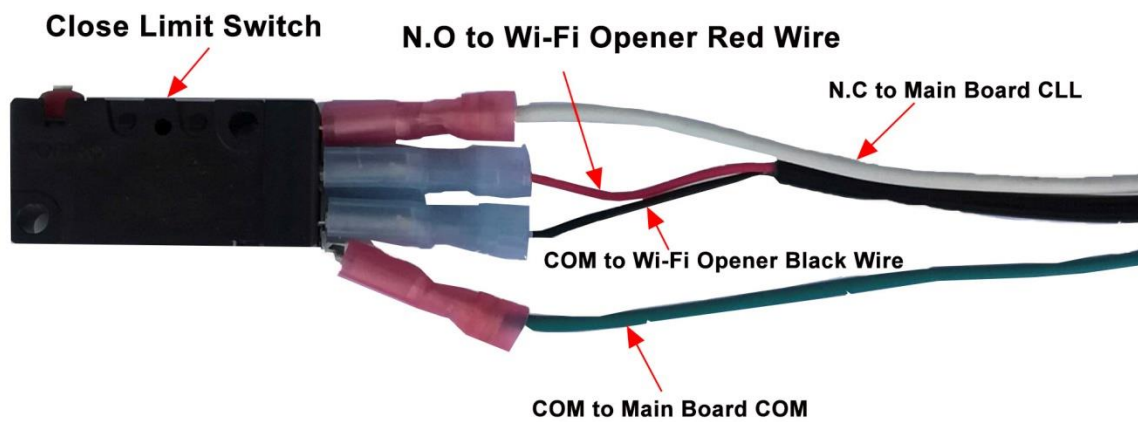
Figure show how to connect Wi-Fi Gate Opener to Close Limit Switch
