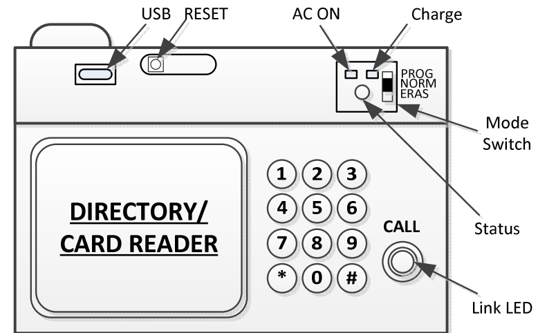
Fig.2 Front Panel
